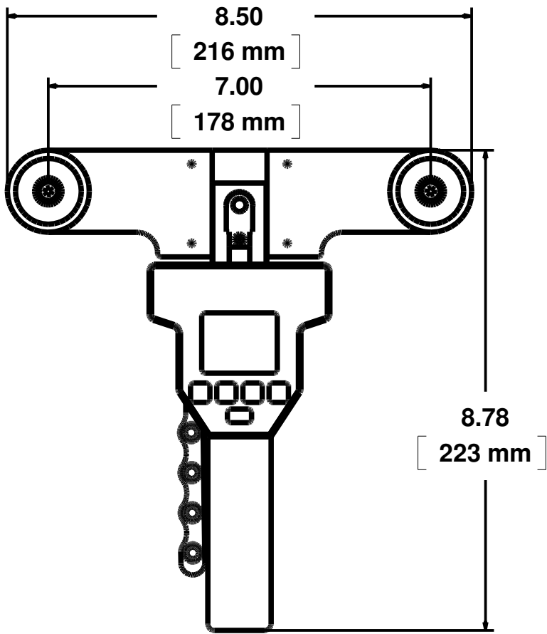
LX-250-W-1 DIGITAL CABLE TENSION METER WITH WIDE FACEPLATE (All Models: LX-250-W-1 and LX-500-W-1)
