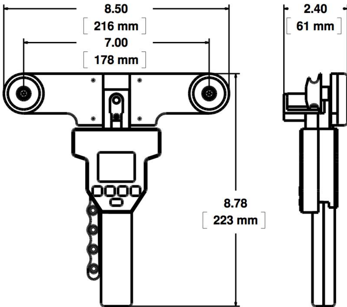
LX-250-W-1 DIGITAL CABLE TENSION METER WITH WIDE FACEPLATE (All Models: LX-250-W-1 and LX-500-W-1)
